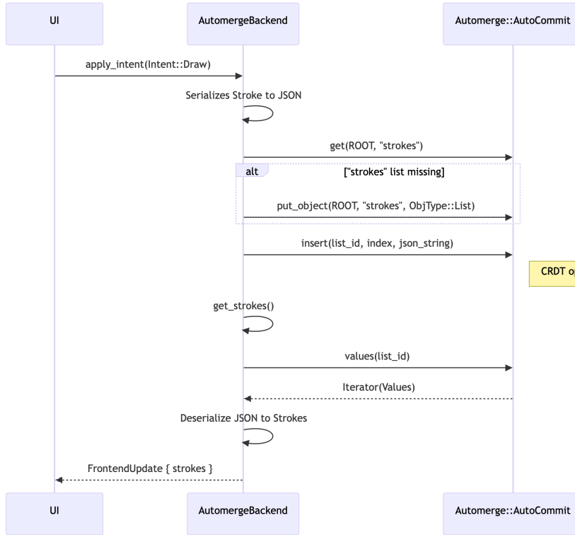
Figure 2.6: Sequence diagram of a local Intent::Draw operation
